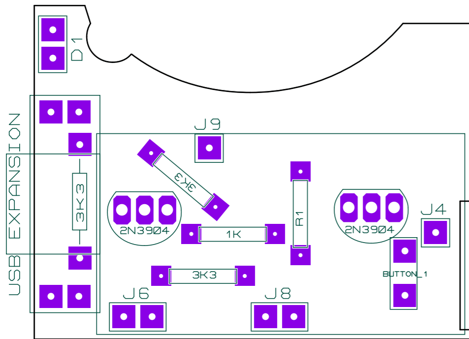
Top Silk
