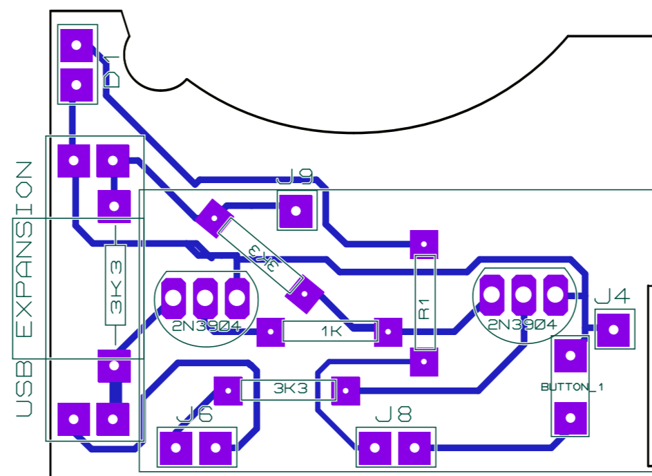
Complete PCB
