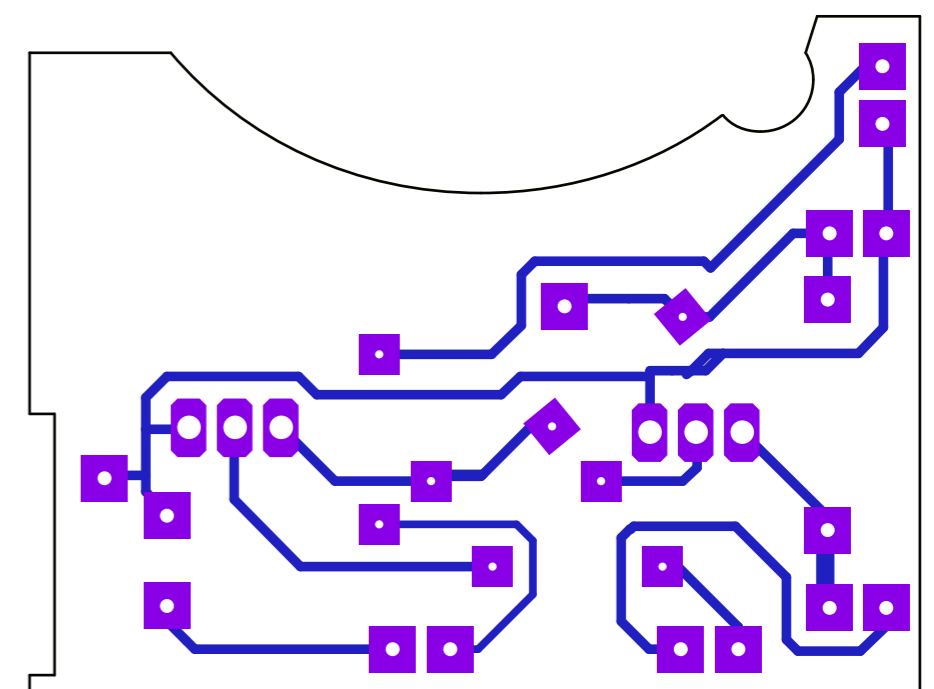
Circuit as seen from PCB bottom
