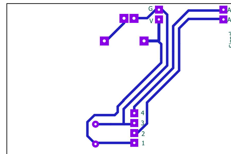
Circuit as seen from PCB bottom
