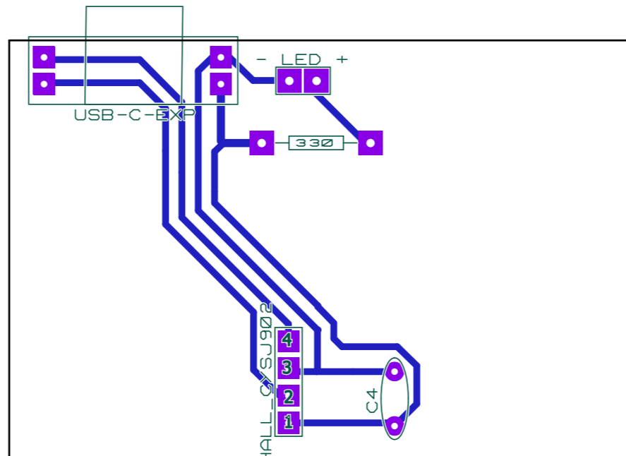
Complete PCB
