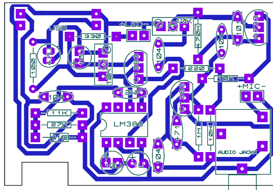
Complete PCB
