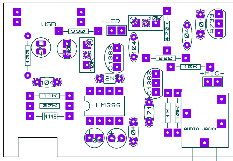
Top Silk
