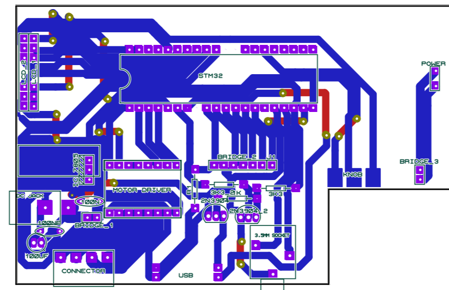
Complete PCB
