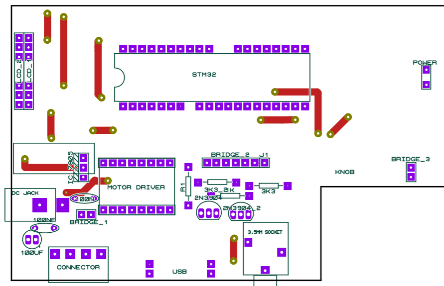
Top Silk
