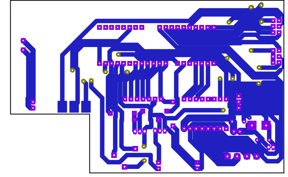
Circuit as seen from PCB bottom
