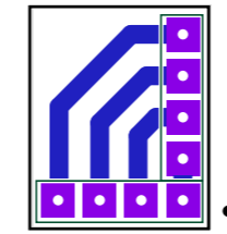
Complete Adapter PCB
