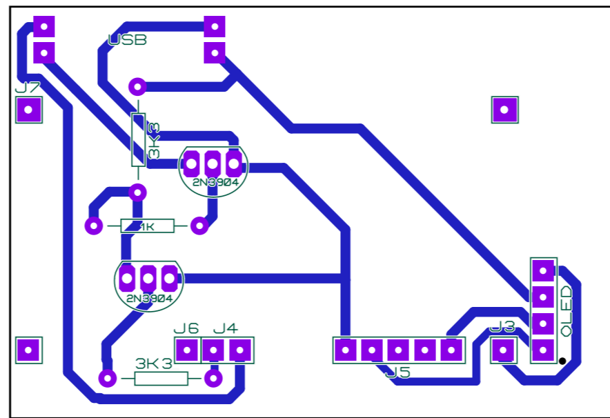
Complete PCB
