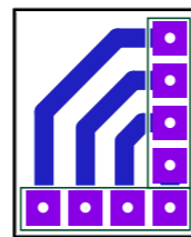
Complete Adapter PCB
